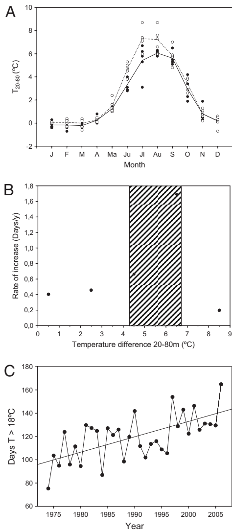
Fig. 2. Main effects of temperature anomaly between depths of 20 m and 80 m on water column stratification. (A) Temperature differences between 20 m and 80 m over the annual cycle during the first 5 years of the series (1974–1978) versus those during the last 5 years (2002–2006), showing the increased intensity in stratification of the water column. (B) Rate of increase (days/year) in the number of days that the temperature difference between 20 m and 80 m was >0.5 – 8.5 °C. The shaded area indicates the range of temperature difference between 20 m 80 m in which the rate of increase was significant (see Table S3). (C) Number of days that temperature was >18 °C at 20 m in 1974–2006.
